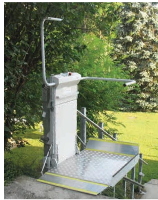
Robust platform mechanics allow for installation in cold or wet environment
